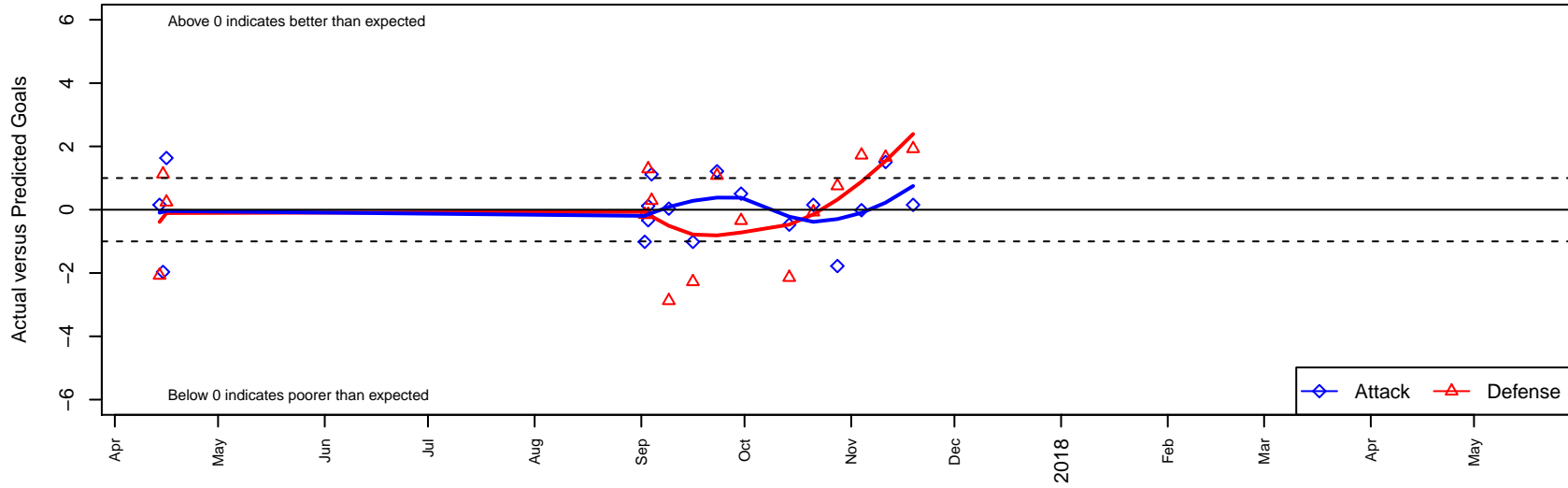
Fusion FC B01 Dots are actual minus expected GF (blue circles) and GA (red triangles). Blue line is smoothed change in attack strength. Red is smoothed change in defense strength.
